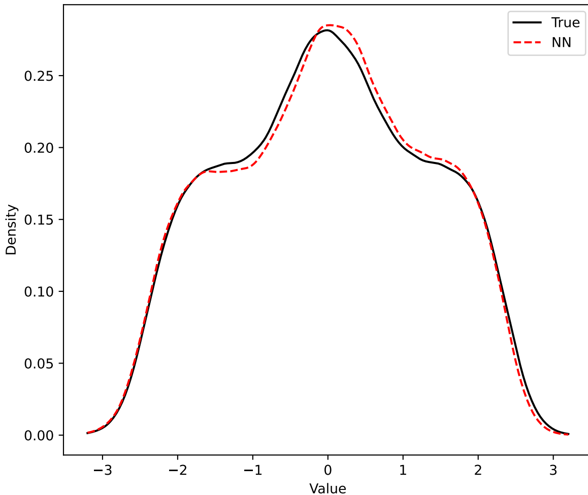
Empirical Density Comparison with KS: 0.0075, p-value: 1.5e-75
