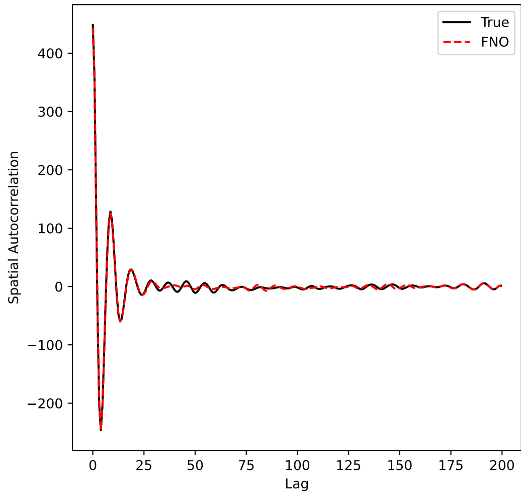
Autocorrelation Comparison with MSE = 8.3
