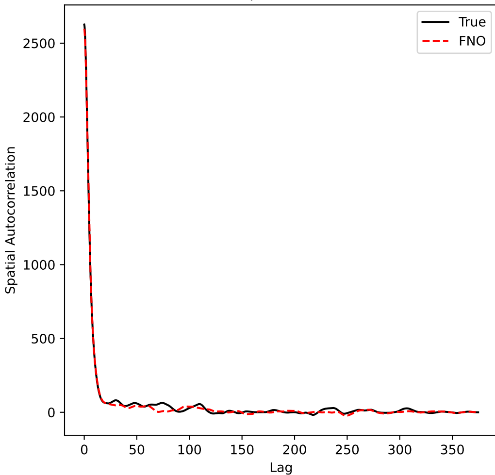
Autocorrelation Comparison with MSE = 2.5 \times 10^2
